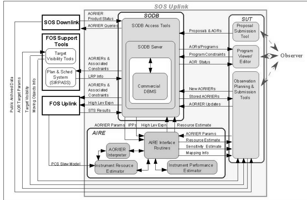
Figure 1. Overview of the SIRTf Uplink Software Design
