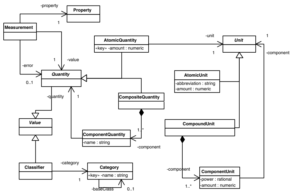
Figure 1. A detail of the domain model, dealing with measurements and values.
