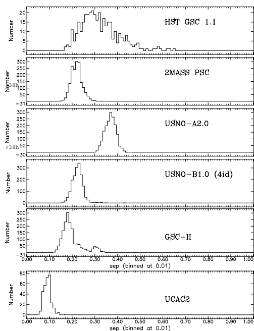
Figure 1. Distribution of image-catalog radial offsets.
